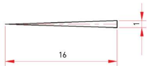
Fig. 3 External thread tapered 1:16
