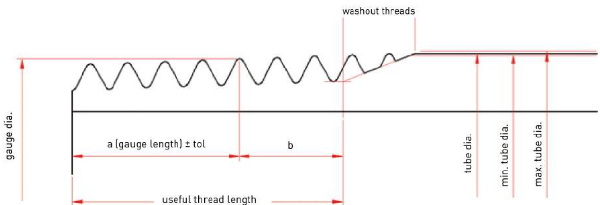
Fig. 2 Taper external thread R on steel tube
